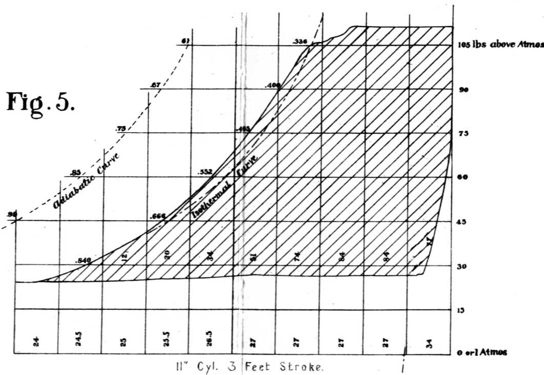
DIAGRAMS from M. Selfe's Compound Compressor.
