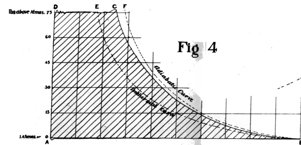
DIAGRAM from a Sommeler Compressor with Hydraulic Piston
