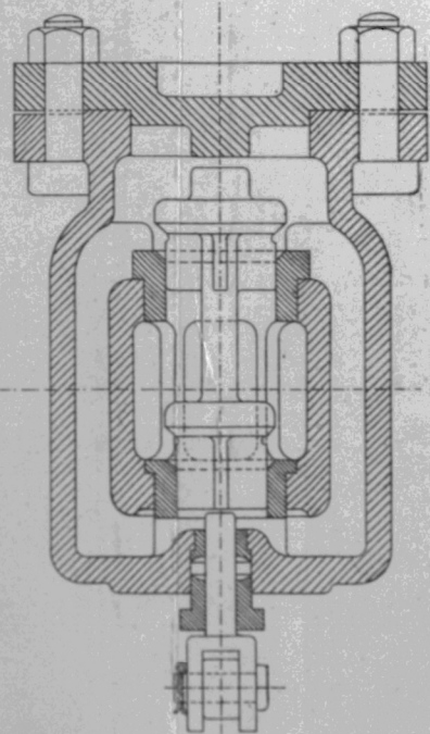
SECTION THROUGH A. B. on Fig. 8.
