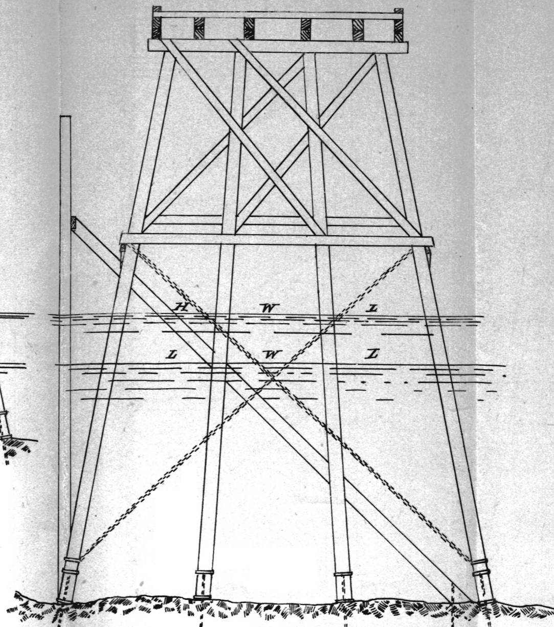
CROSS SECTION AT C.C.
