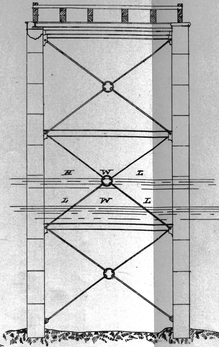
CROSS SECTION AT D.D.
