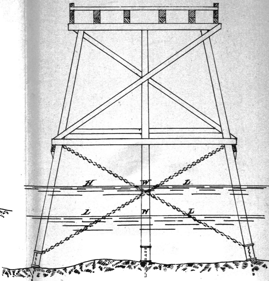
CROSS SECTION AT B.B.
