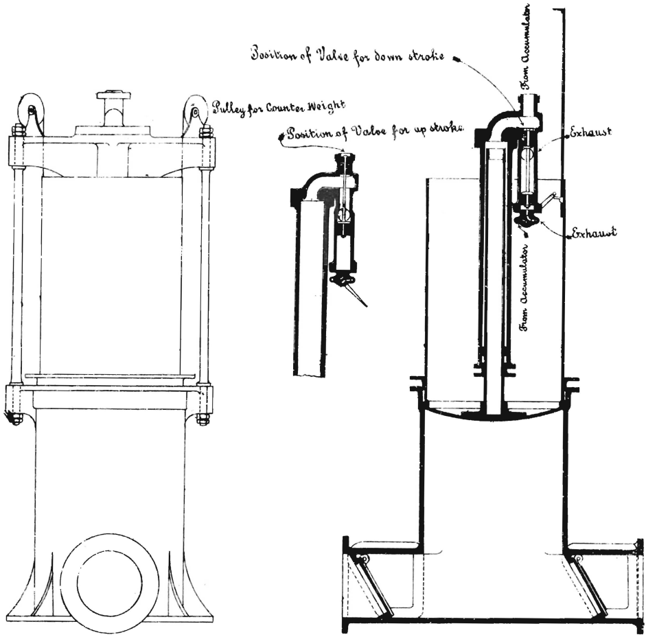
APPLEBY'S HYDRAULIC SEWAGE LIFTER
