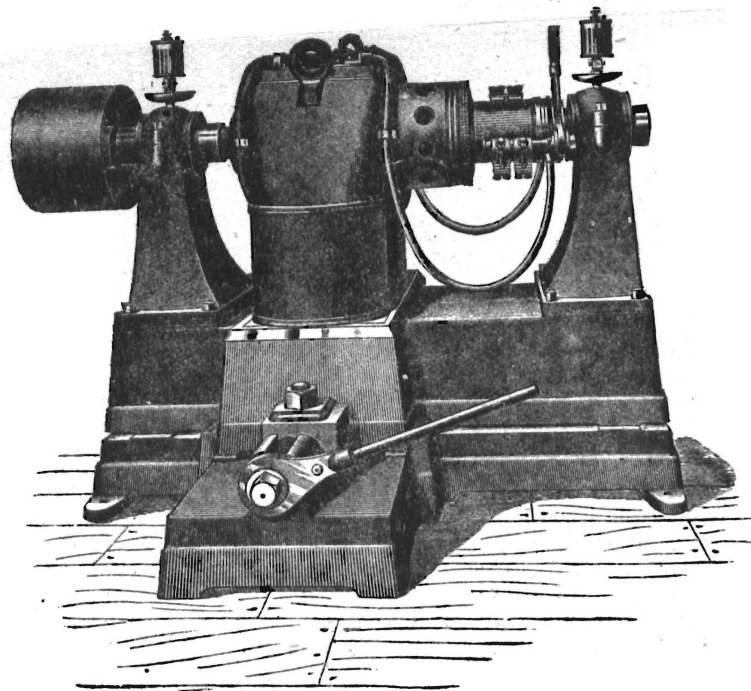
40,000 WATT MOTOR TYPE DYNAMO.
