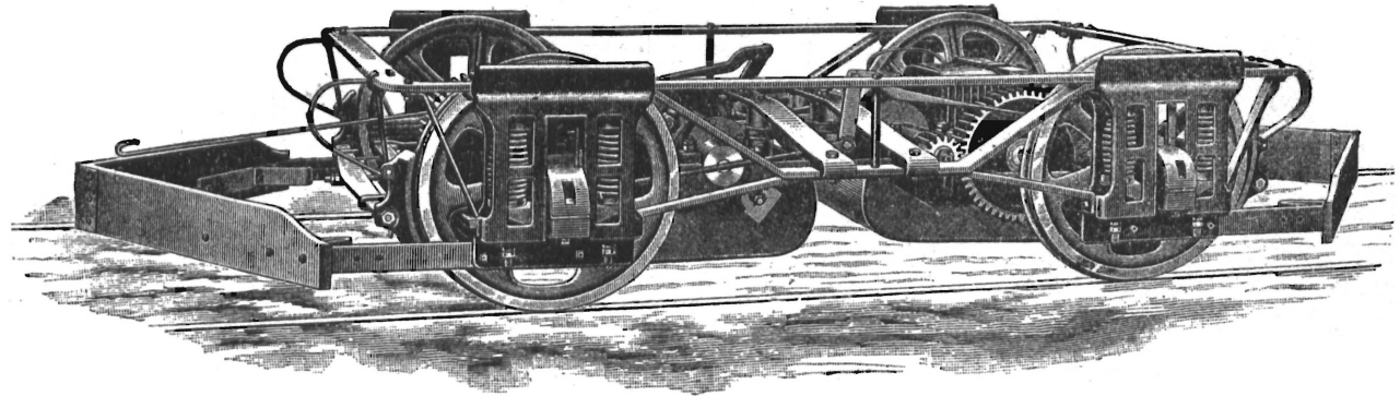
NEW TYPE THOMSON-HOUSTON ELECTRIC RAILWAY TRUCK.
