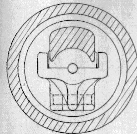
TRANSVERSE SECTION AT XX
