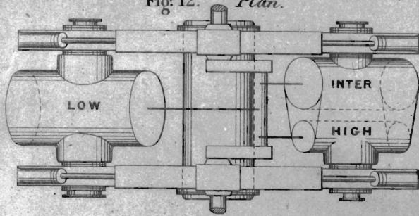
Rodger's Oscillating Engine.
