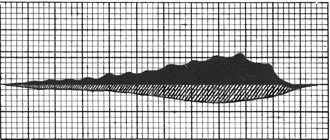
INDICATOR DIAGRAM, FIG. 1. JOINT ABOVE ZERO EQUALS DEFLECTION OF JOINT AT X. ETCHING BELOW ZERO SHEWS SLEEPER DEPRESSIONS.
