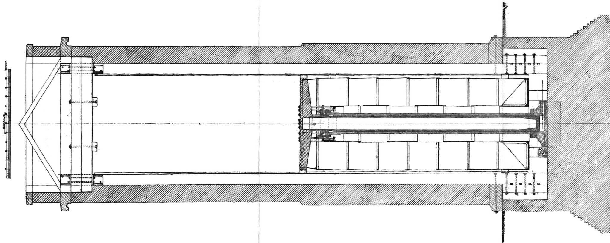
PLAN & SECTION OF ACCUMULATORS.
