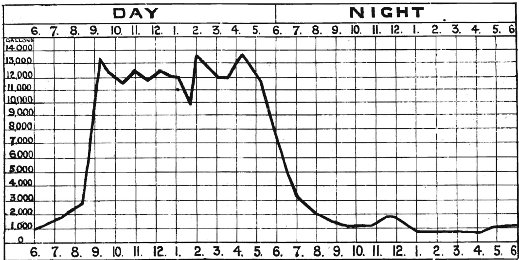
DIAGRAM SHOWING QUANTITY OF WATER PUMPED PER HOUR DURING AN ORDINARY WORKING DAY.
