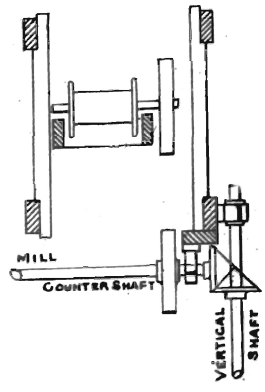
FROM A DRAWING MADE BY THE AUTHOR FOR FLOUR MILL FOR TUMUT N.S.W. (SIGNED) SUSSEX ST ENGINE WORKS FEB. 28 TH 1856.
