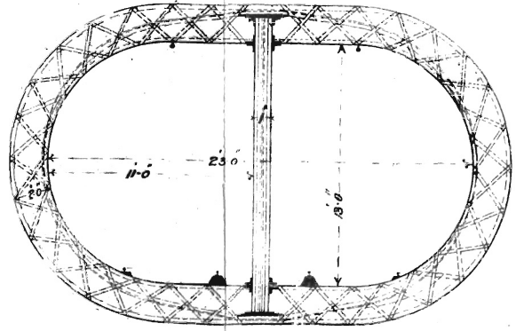
ENLARGED SECTION of VIADUCT.
