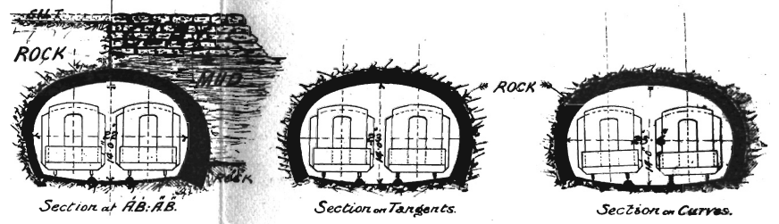
Cross Sections of Tunnels.
