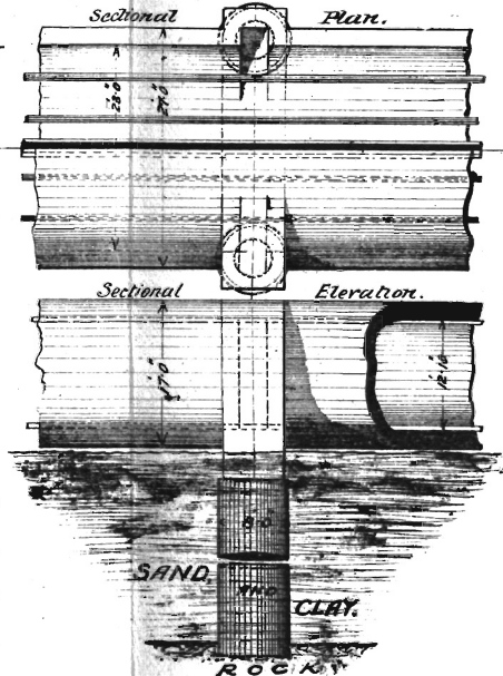
PLAN of SUBMERGED BRIDGE
