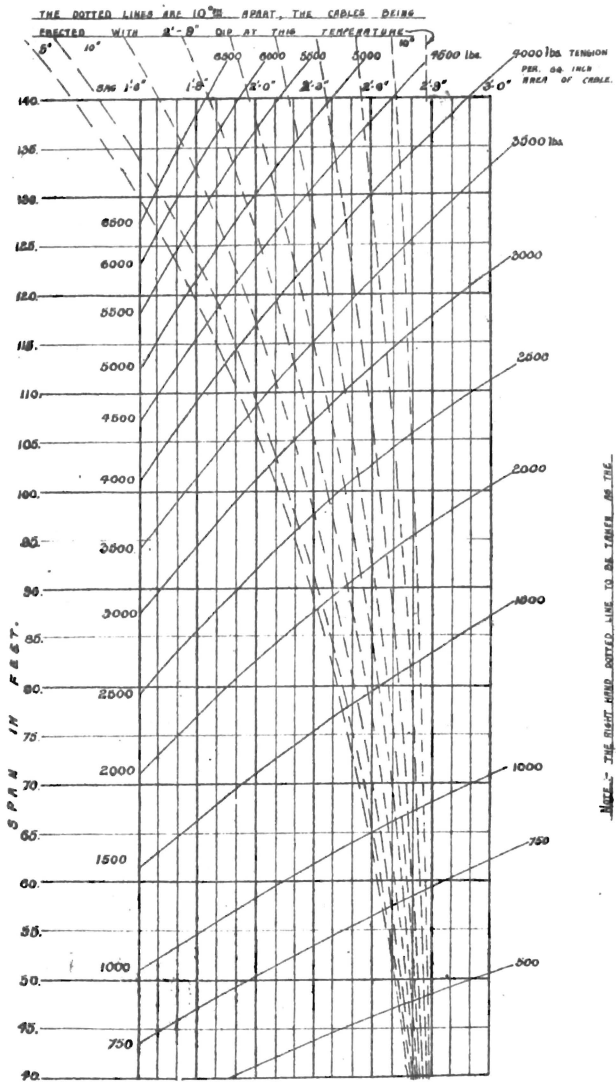
DIAGRAM SHEWING THE VARIATION IN DIP AND STRESS OF COPPER CABLES DUE TO CHANGES OF TEMPERATURE FOR SPANS FROM 40 FT TO 140 FT
