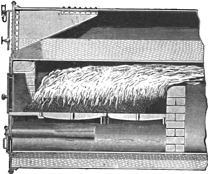
Longitudinal Section through Furnace.
