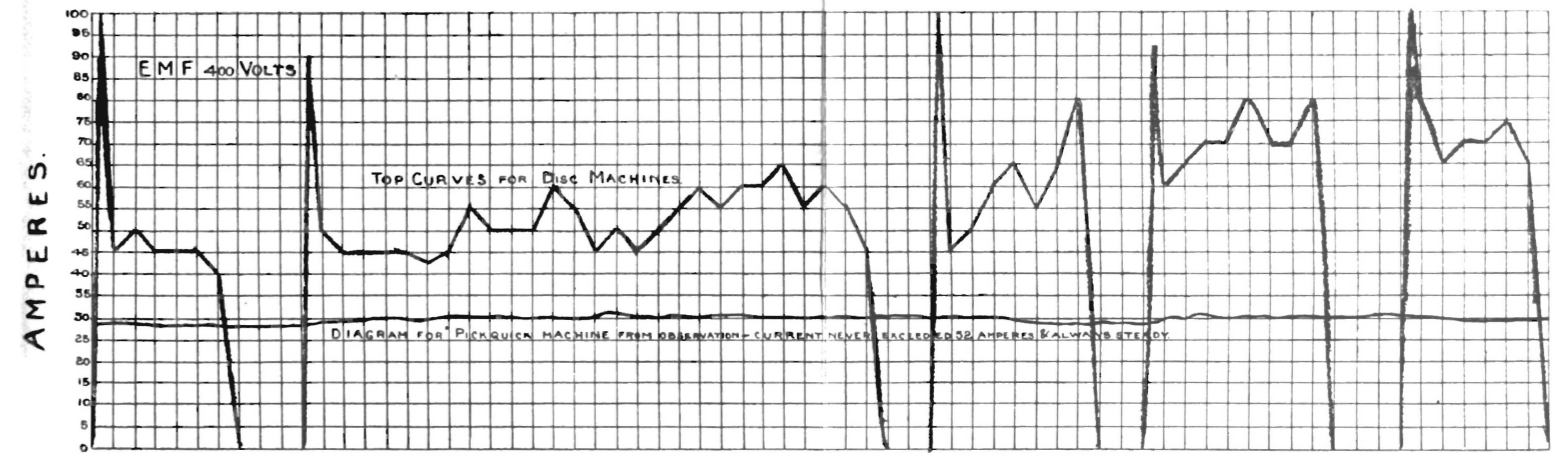
COMPARATIVE LOAD DIAGRAMS OF BAR & DISC MACHINES.
