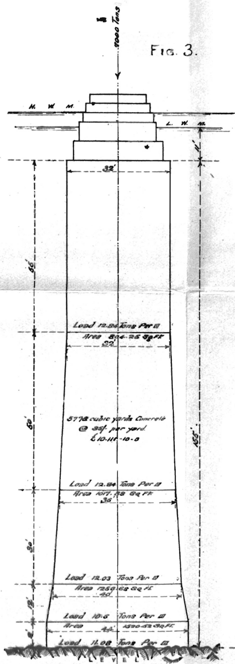
PIER WITH UNIFORM LOADING THROUGHOUT
