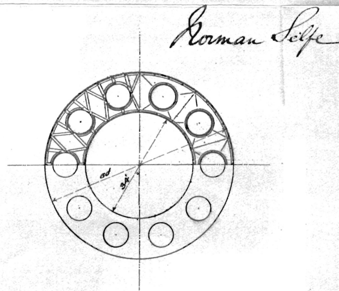
ANNULAR PIER IN CAISSON
