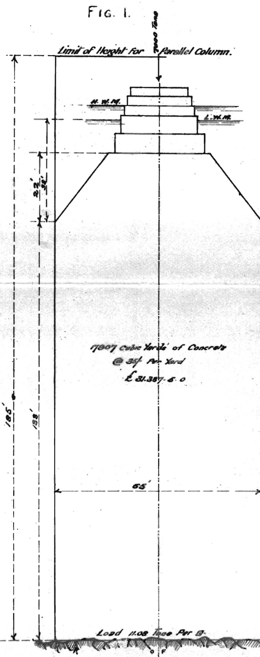
SOLID PIER IN PARALLEL CAISSON
