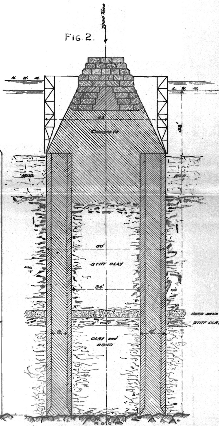
ANNULAR PIER IN CAISSON
