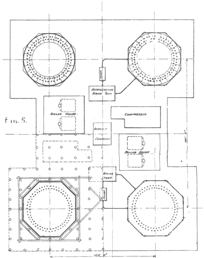
GENERAL PLAN OF WHARF AND THE FOUR FOUNDATIONS TO NORTHERN GREAT PIER
