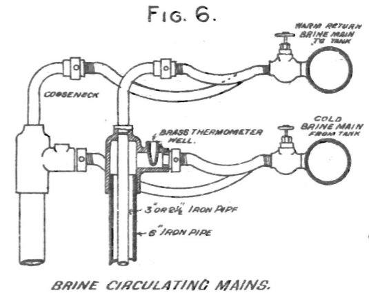
BRINE CIRCULATING MAINS.
