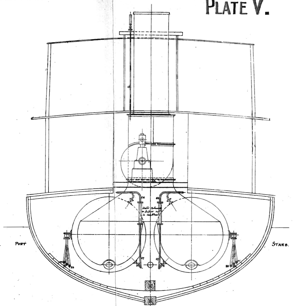
AFT END OF BOILERS — LOOKING FORD.
