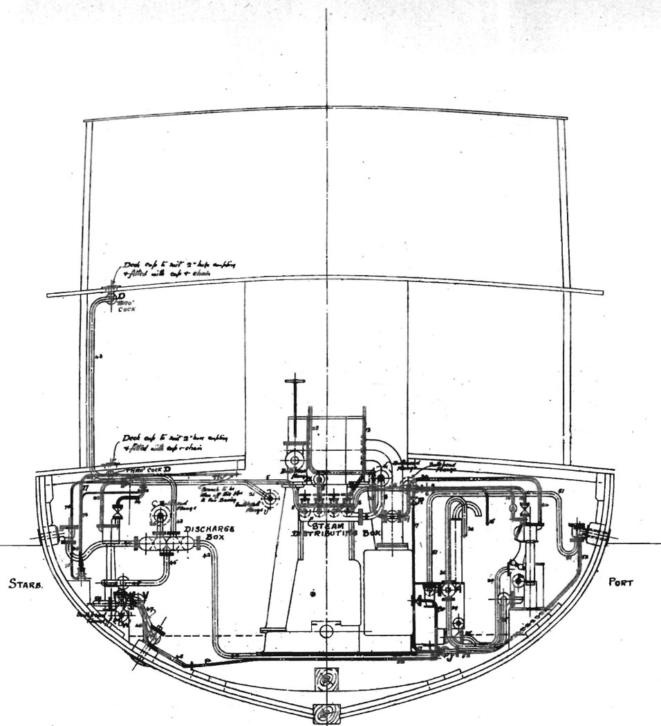
FORD END OF ENGINE ROOM — LOOKING AFT
