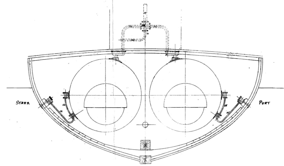
FORD END OF BOILERS — LOOKING AFT
