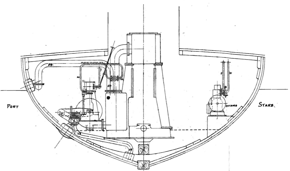
AFT END OF ENGINE ROOM — LOOKING FORD
