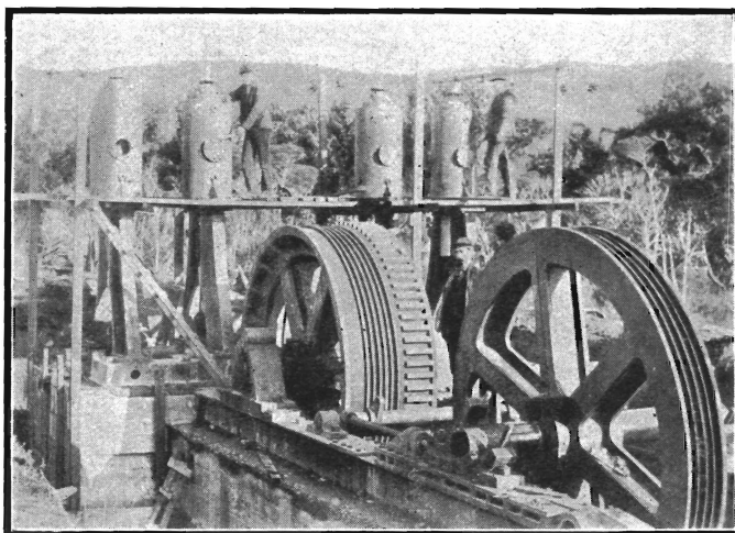
View of Hydraulic Brakes—No. J.
