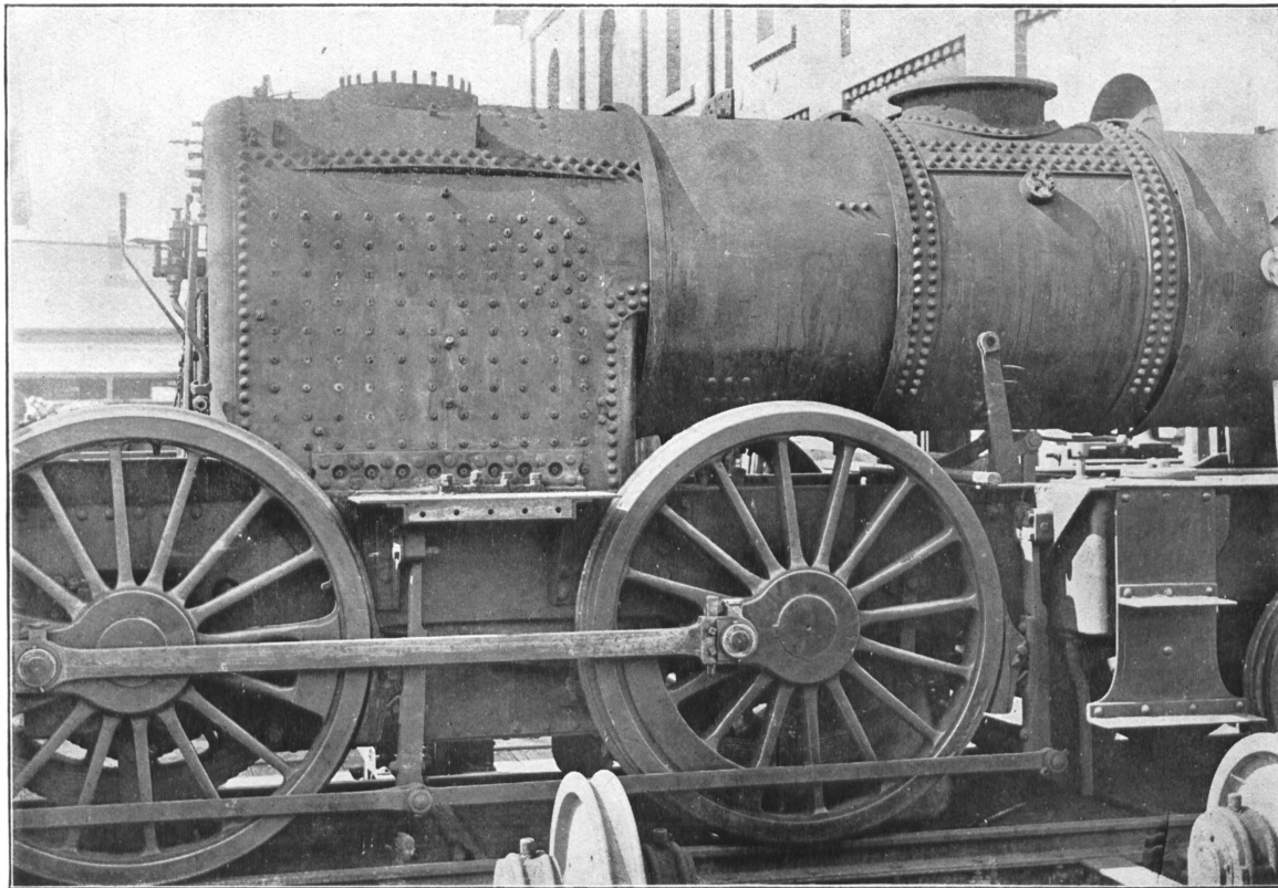
FIG 1A—Side View of Boiler No. 163.
