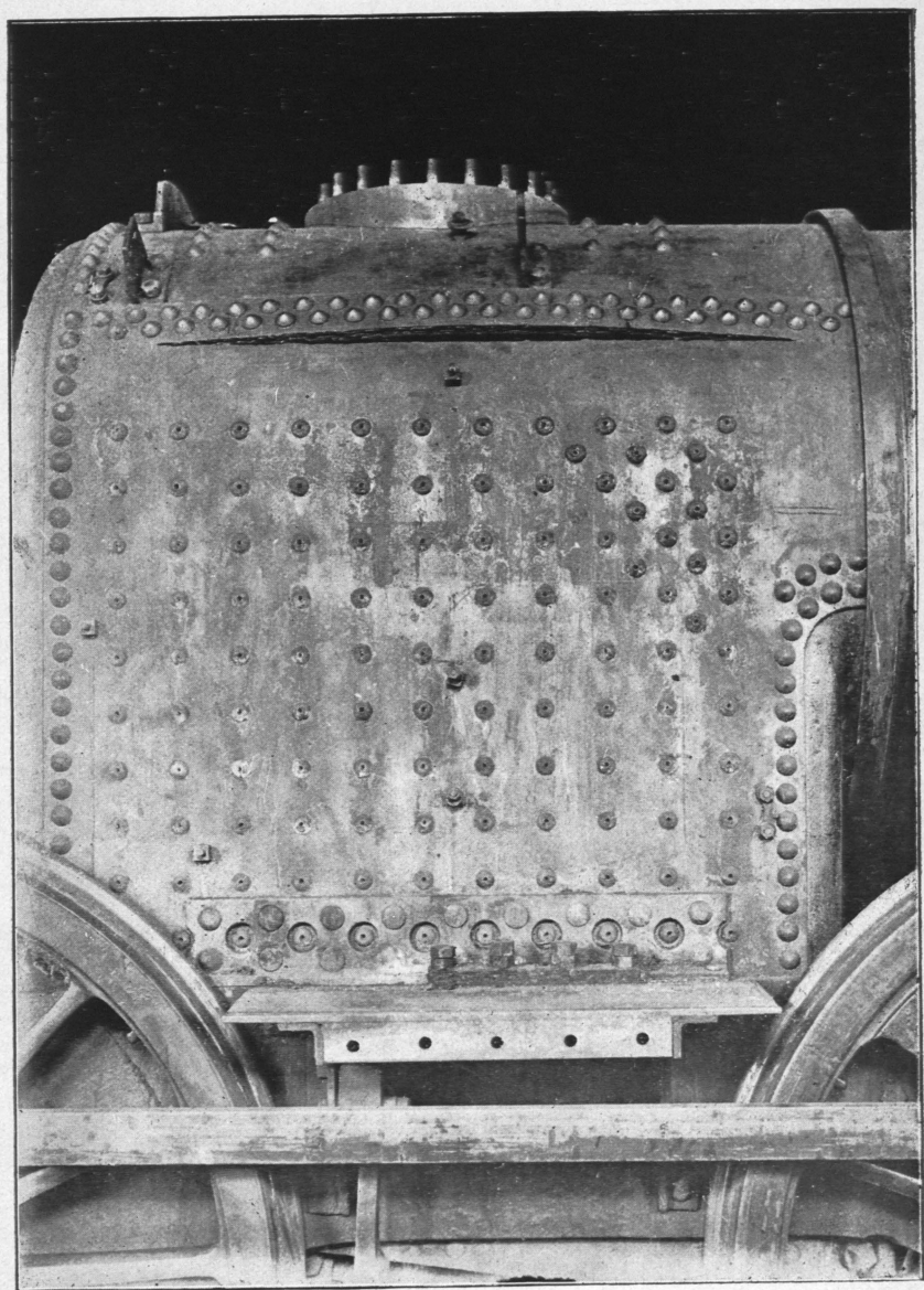
FIG 1B.—Near View of Fractured Plate.
