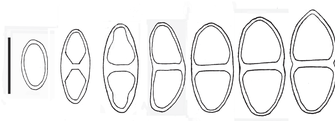
Fig. 5. Ascospore ontogeny of B. maungatuensis . Scale = 10 \mu m.
